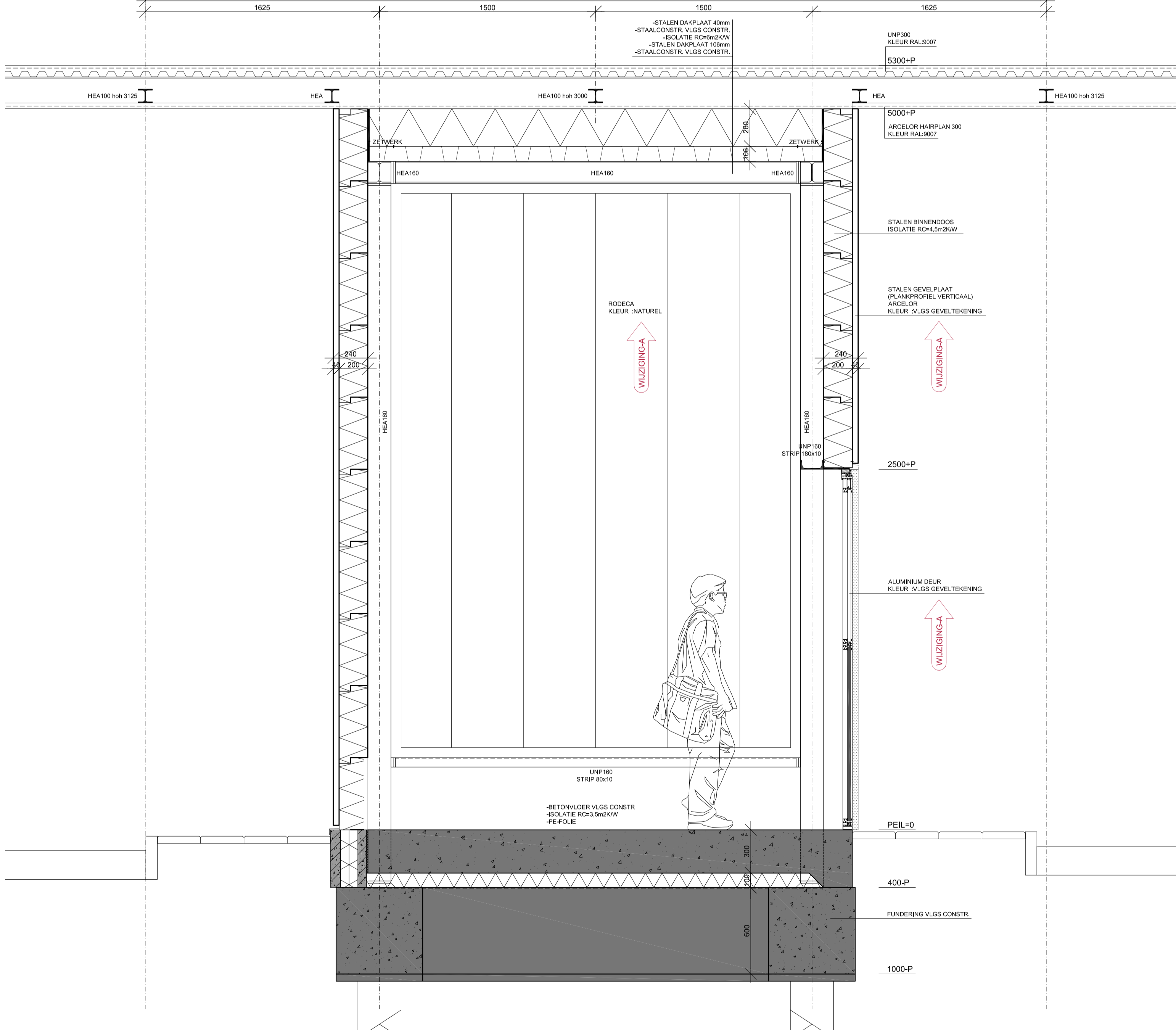
DETAIL V-02
