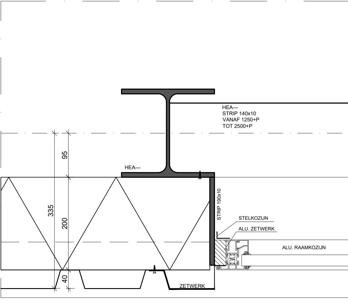
DETAIL H-05
