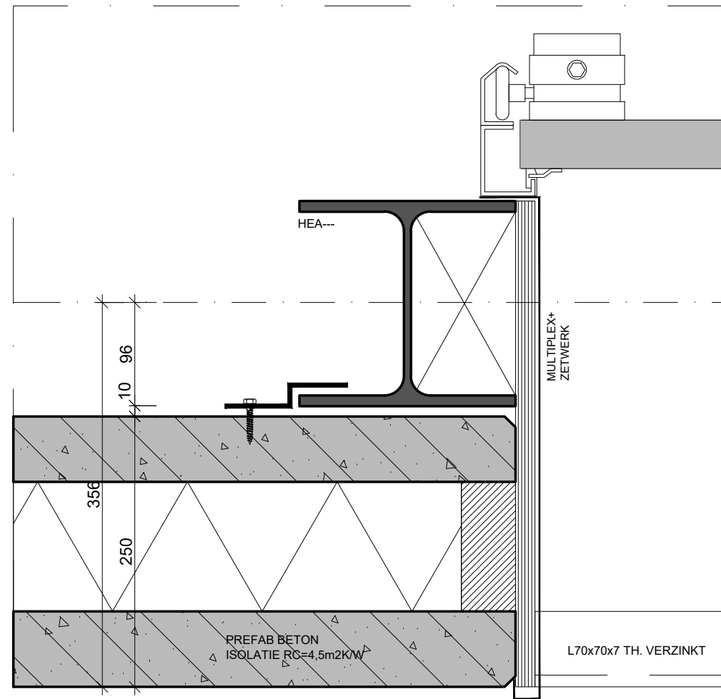
DETAIL H-01
