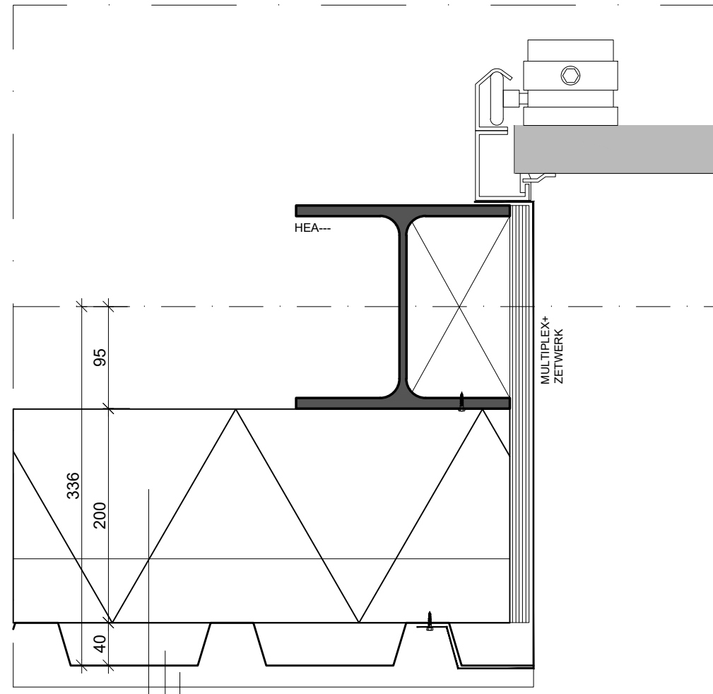
DETAIL H-02
